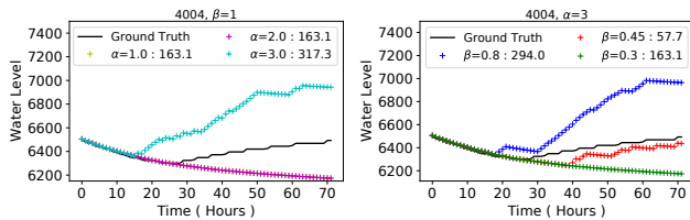
Figure 6: Loss function parameter choices for sensor 4004.
