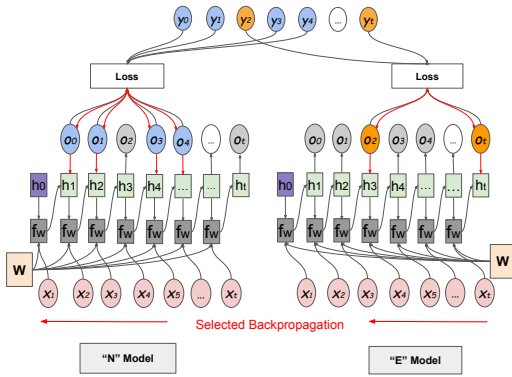
Figure 4: Computational graph for the N and E models. Blue and orange inputs represent normal and extreme values, respectively.
