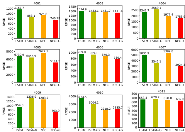
Figure 5: Effectiveness comparison of NEC and LSTM variants with (LSTM+G and NEC+G) and without (LSTM and NEC) GMM indicator variables across all 9 sensors.
