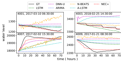
Figure 7: Example 3 days ahead predictions for four sensors.
