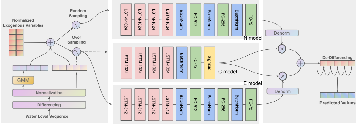
Figure 2: The NEC+ framework; \oplus denotes the element-wise addition and \otimes denotes the element-wise product.
